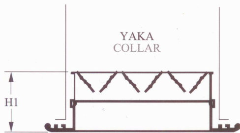
ZIT KANATLI DAMPER OPPOSED BLADE DAMPER
